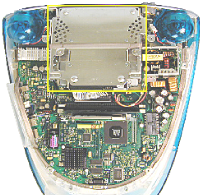
CD/HD Carrier
