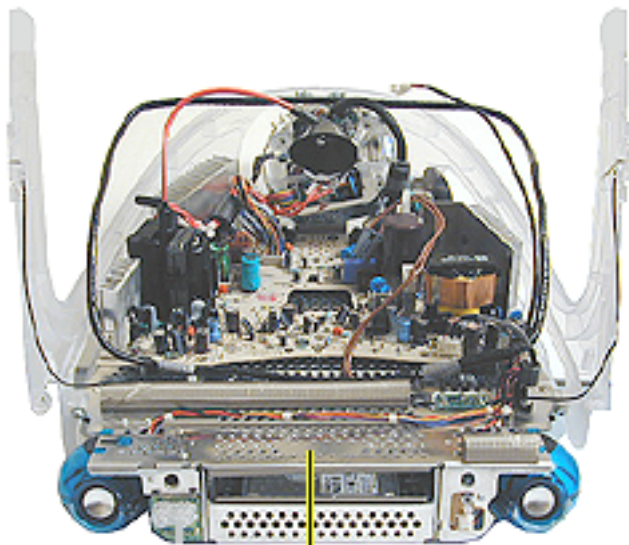
Divider Panel
